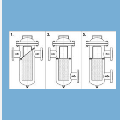
Basket Filter Housing
